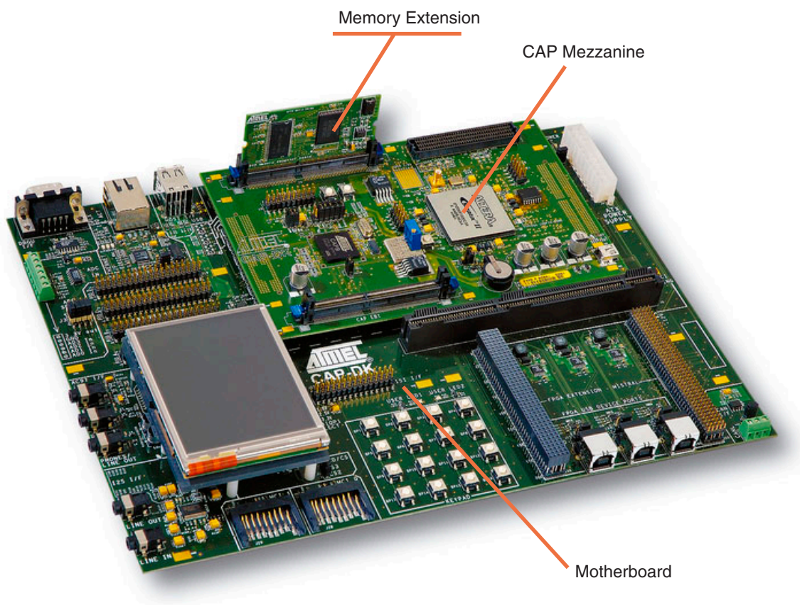
Figure 12-1. AT91CAP-MEM33 Overview
